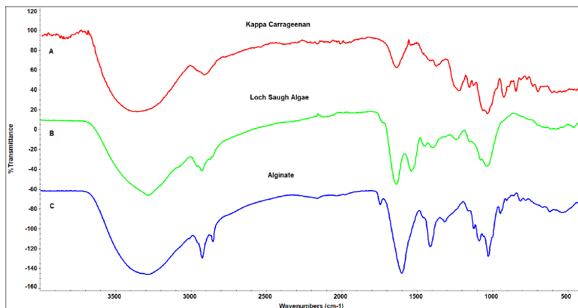
Figure 13. FT-IR spectra of some marine products.
