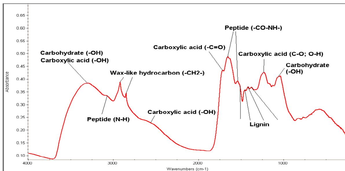
Figure 10. IR spectrum of mineral soil humic acid.
